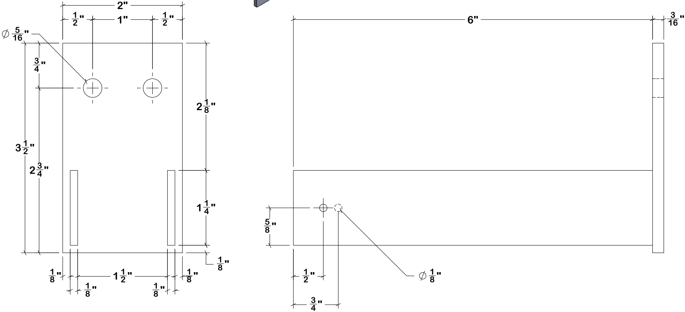
SC15.3-B Original 1 1/2" Bottom Saddle Clip with (2) 1/4" Ø SDS Screw & (2) 1/4" TEK Screws
