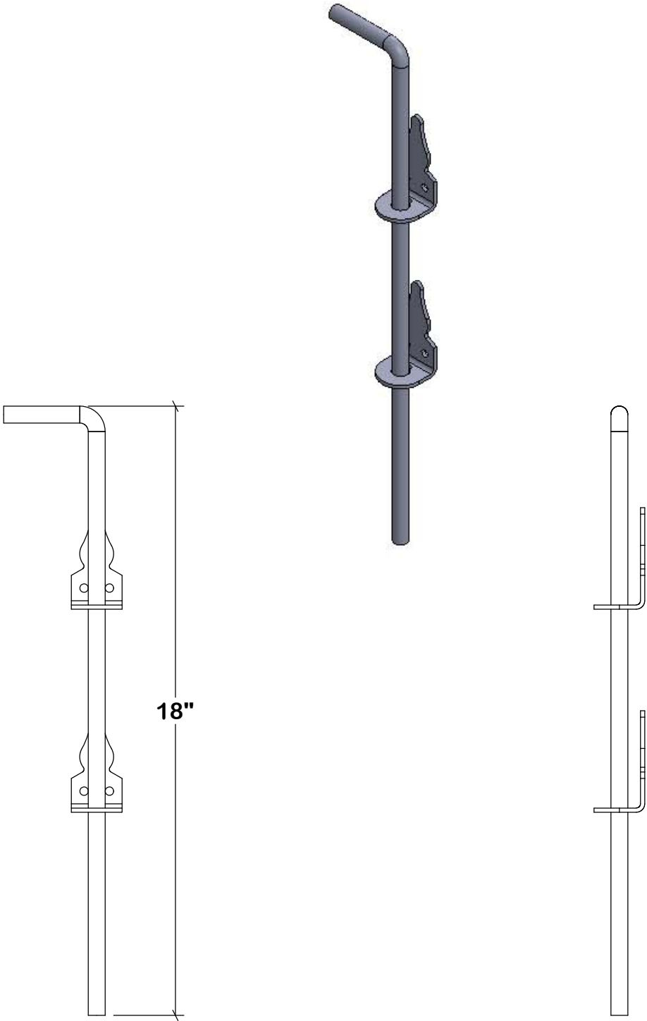
Cane Bolt Assembly (4) 1/4" Ø TEK Screws Ordered Part ###
