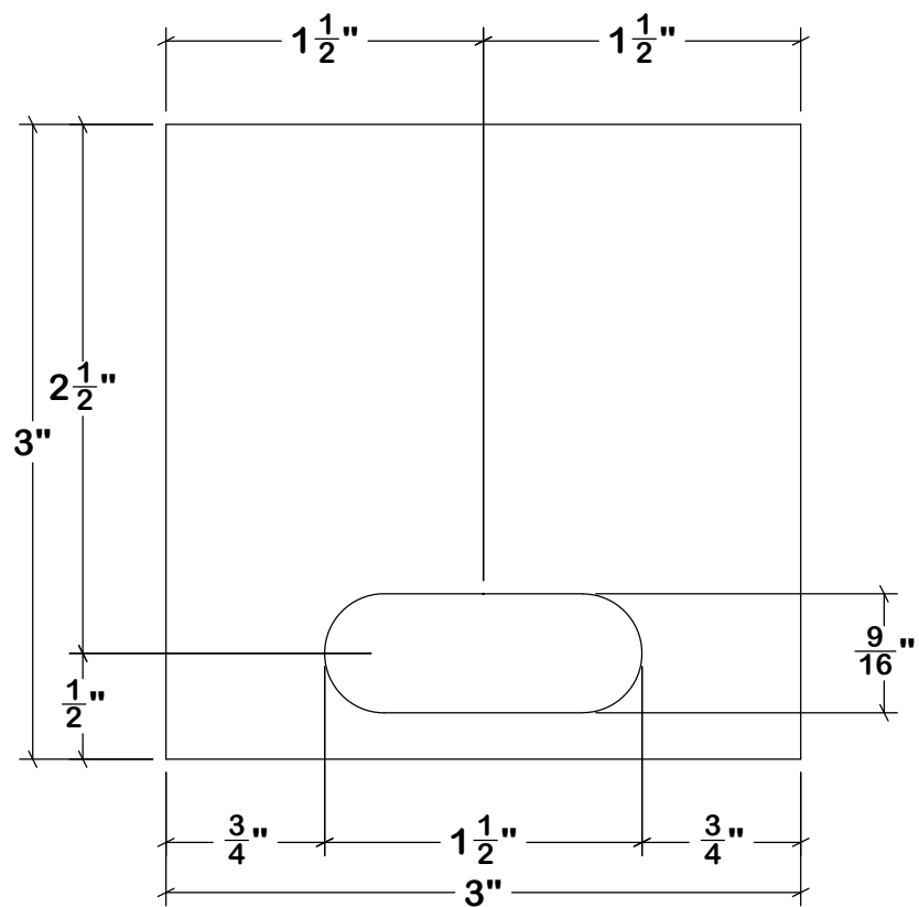
SPB Stringer Bottom Plate (1) 1/2" Ø Wedge Anchor / Lag Bolt
