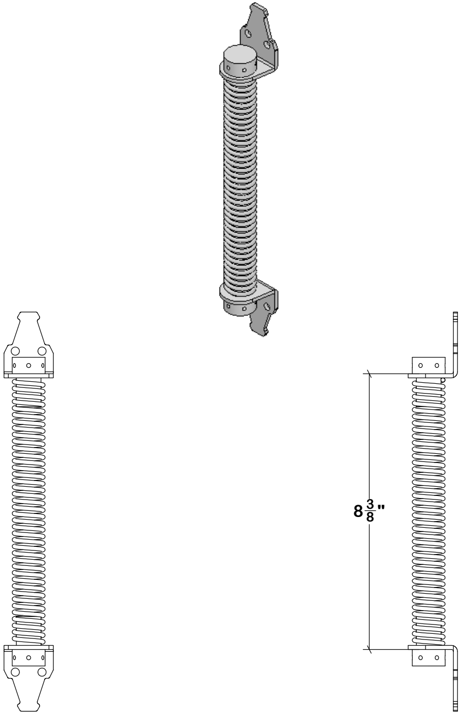
Typ. Spring Closure (4) 1/4" Ø TEK screws Ordered part From ###
