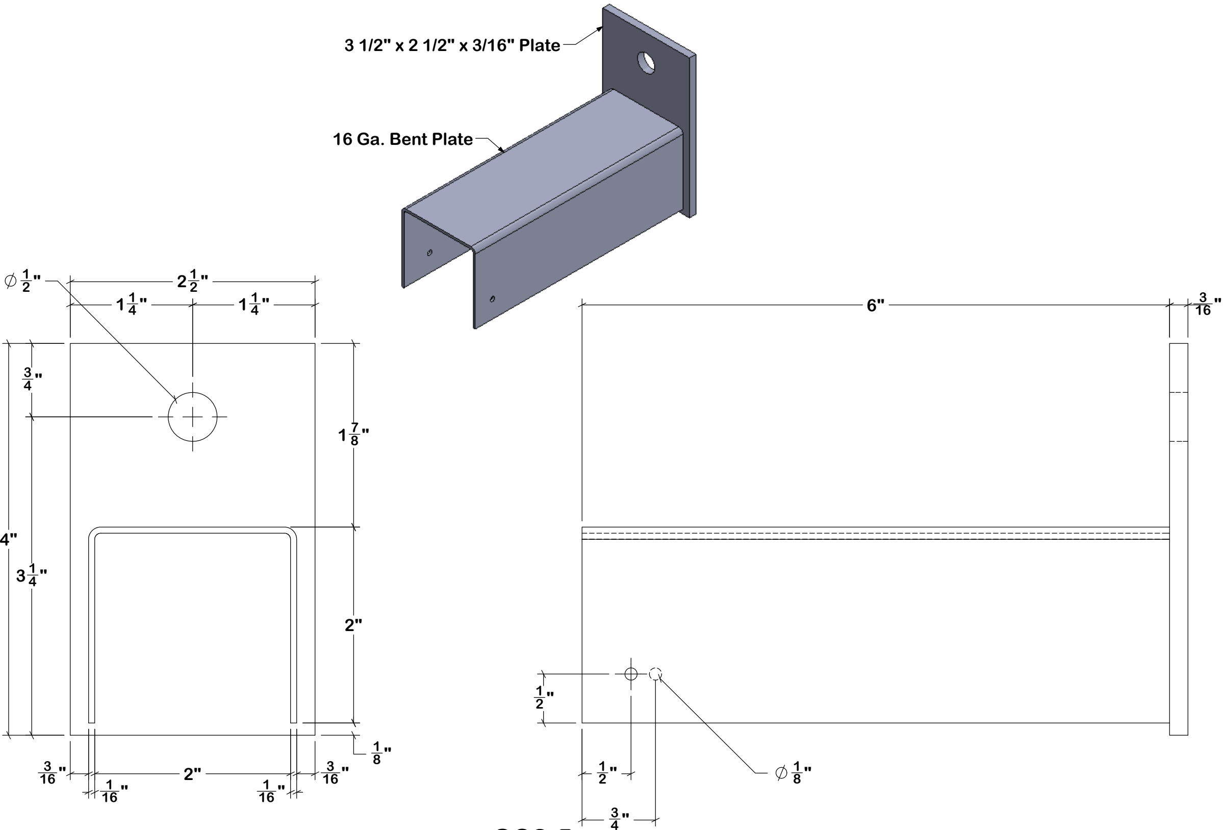
SC2.5 Original 2" Saddle Clip with (1) 3/8" Ø Lag/ HD Titen Bolt & (2) 1/4" TEK Screws
