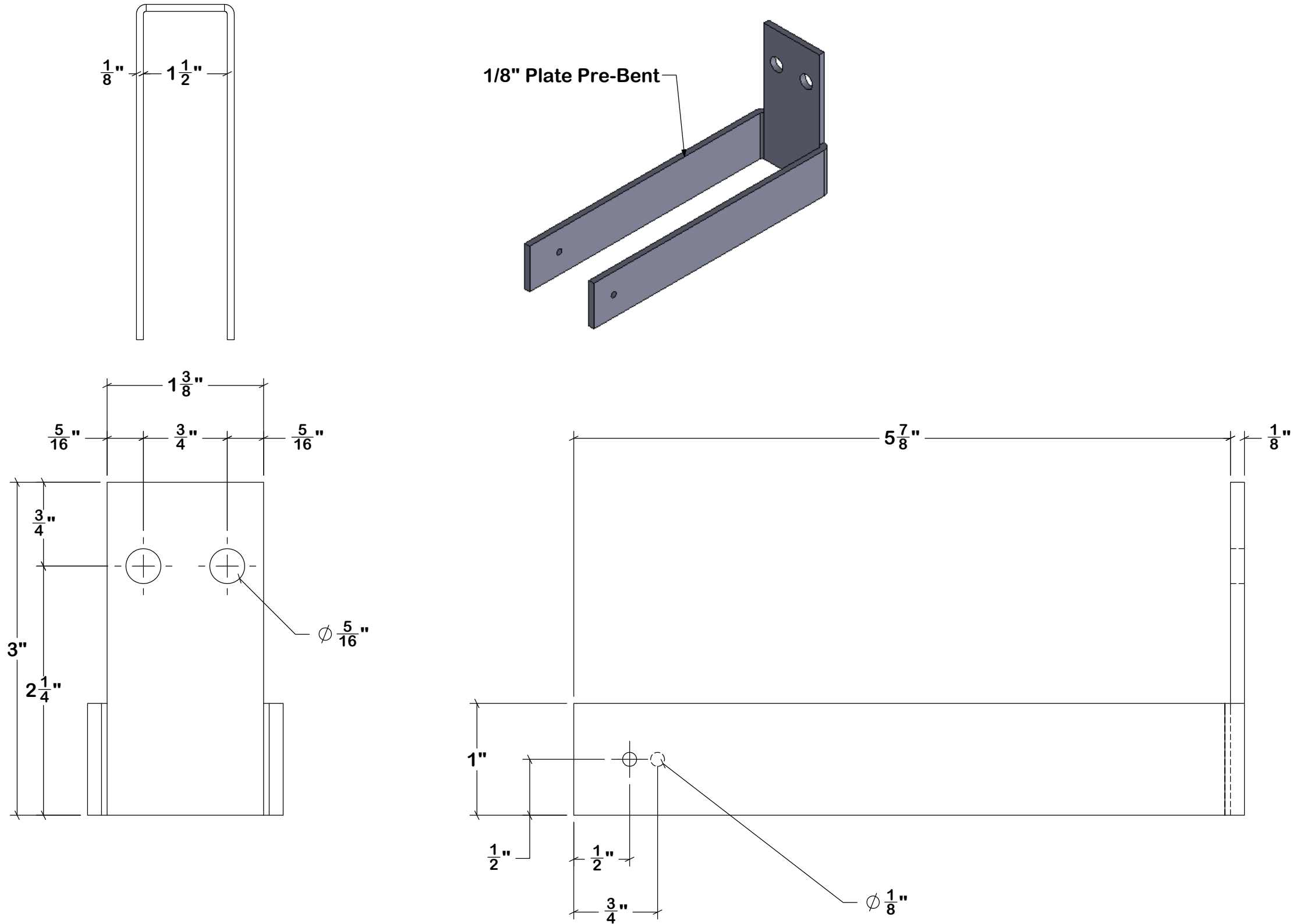
Typ. Bent Bottom Plate - 1 1/2" Tube (2) 1/4" Ø SDS Screws & (2) 1/4" Ø TEK Srews
