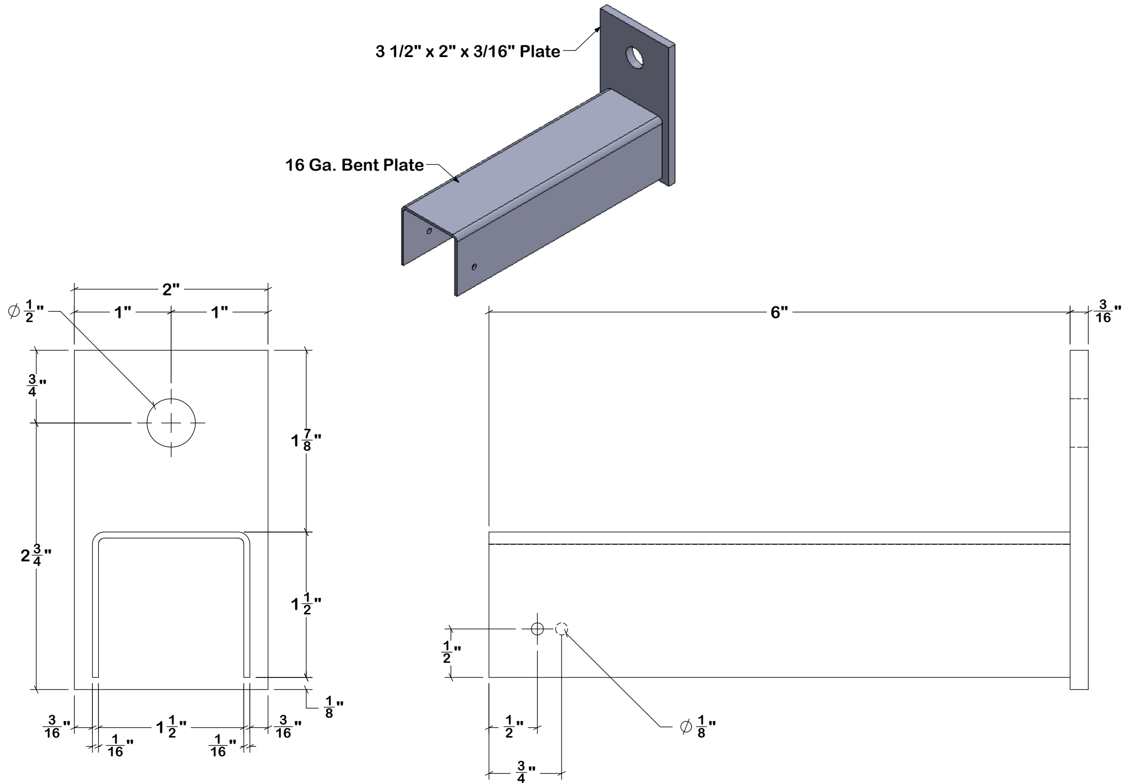
SC15.5 Original 1 1/2" Saddle Clip with (1) 3/8" Ø Lag/ HD Titen Bolt & (2) 1/4" TEK Screws
