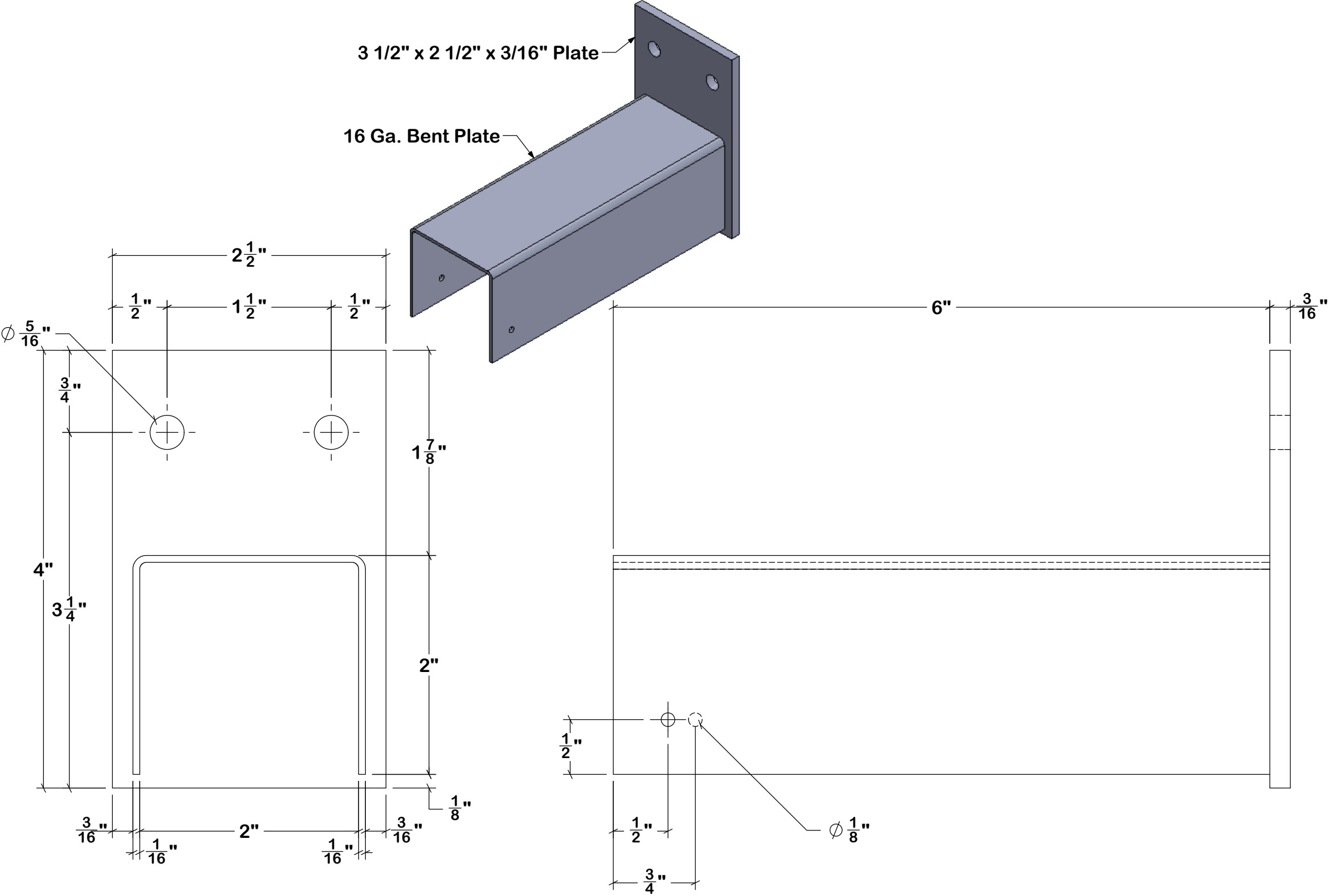
SC2.3 Original 2" Saddle Clip with (2) 1/4" Ø SDS Screws & (2) 1/4" TEK Screws
